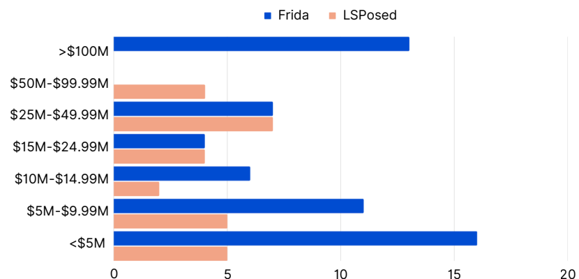
Hooking framework results by annual revenue (in %)
